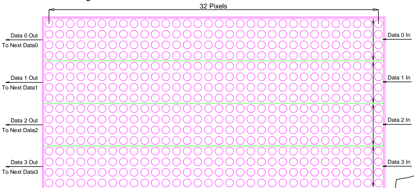
FRONT VIEW (LAMP VIEW)
