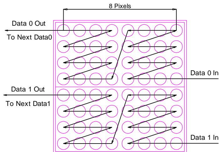
FRONT VIEW (LAMP VIEW)
